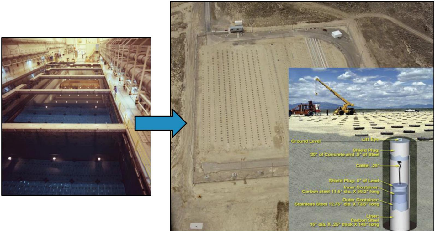
Figure 23: Wet storage (left) and dry cask storage (right) of EBR-II SNF at INL 82
